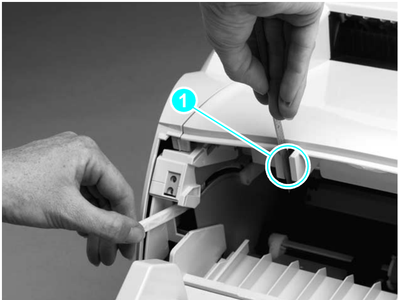
Figure 59. Override SW301
