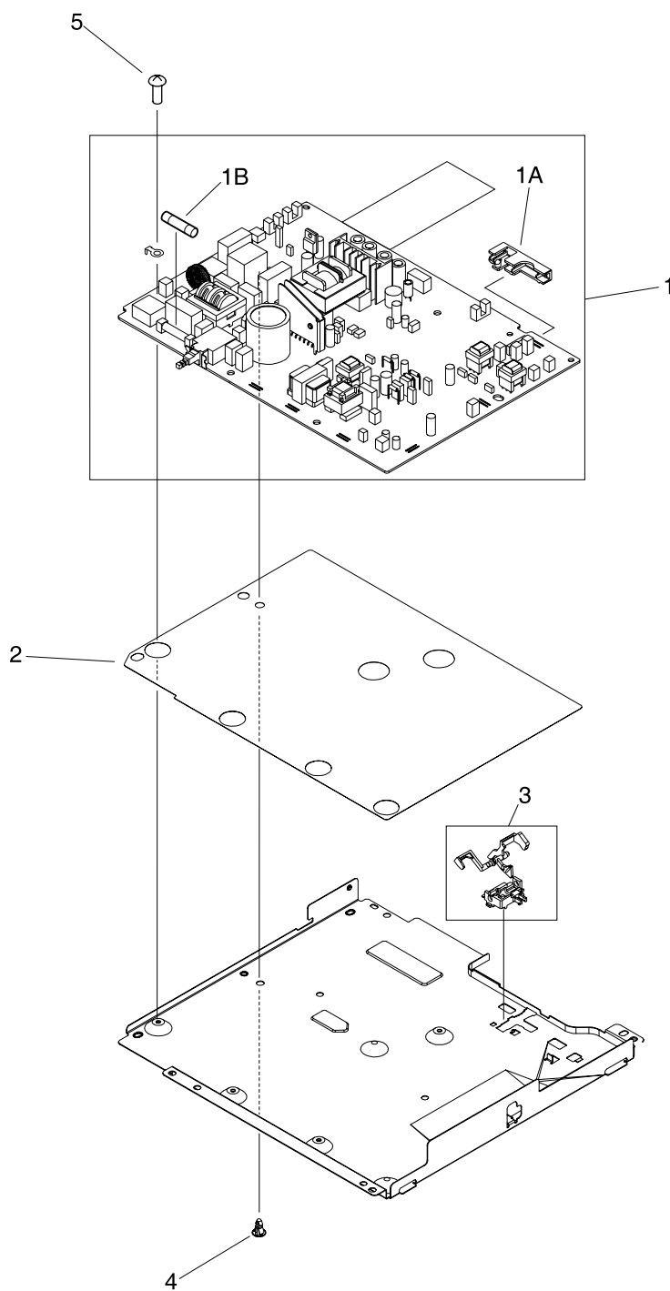
Figure 129. Power-supply assembly
