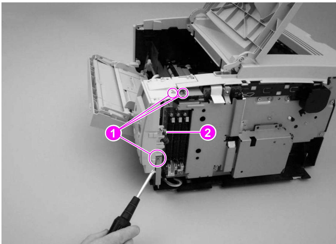
Removing the control panel
