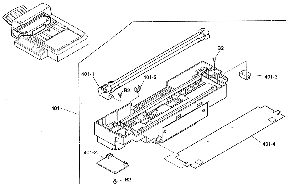
Figure 8-22 Carrier Unit
