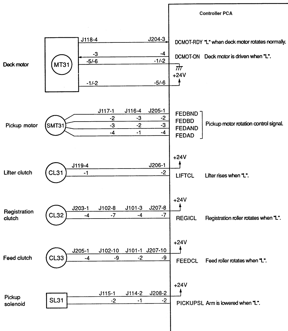
Figure 7-34 2000-sheet Input Tray Controller PCA Outputs
