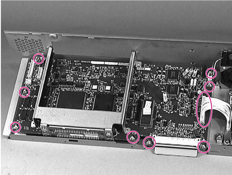
Figure 6-223 Control PCA
