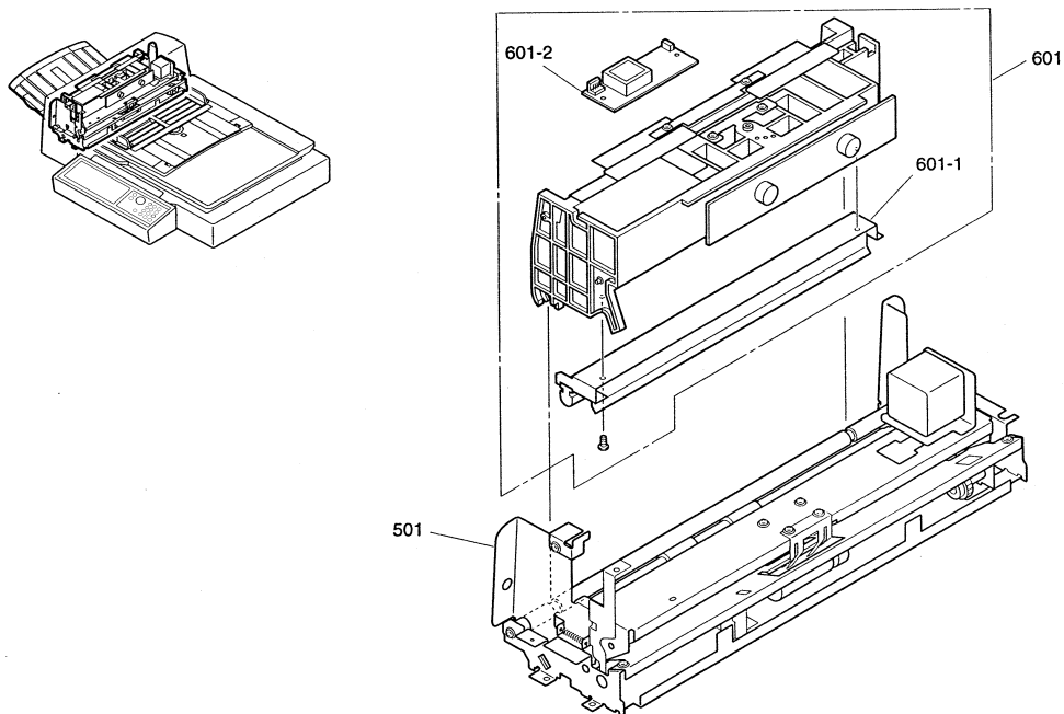
Figure 8-24 Optical Unit
